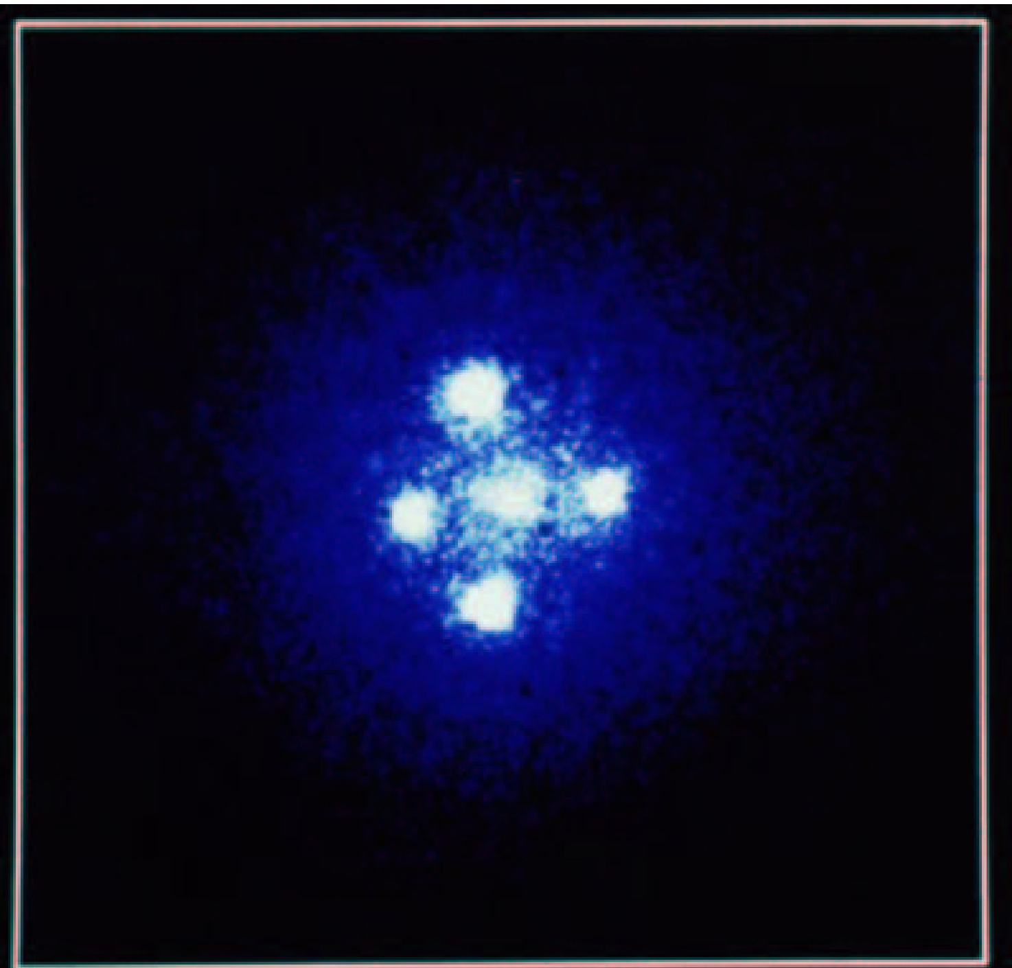
Gravitational Lens G2237+0305
