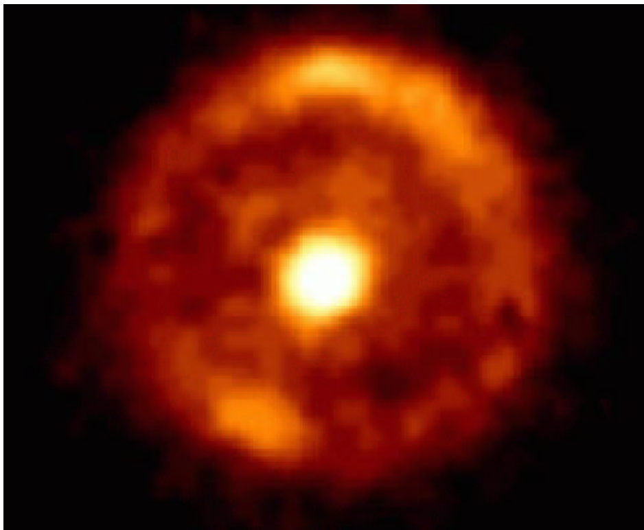
Figure 12.3: Hubble Space Telescope image of an Einstein ring, where a fortuitous alignment has caused an intervening elliptical galaxy to lense a background spiral galaxy into a ring.
