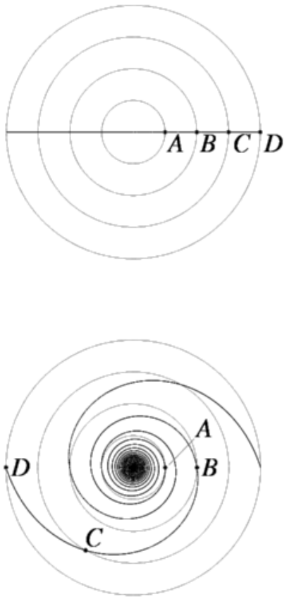
Figure 5.2: A spiral pattern made out of stars will rapidly wind-up in a disk undergoing differential rotation.
